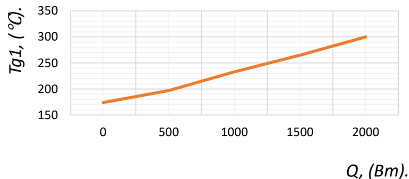
Figure 2. The dependence of the temperature of exhaust gases from the engine ( T_{g1} ) on the load (N) applied to the engine.
